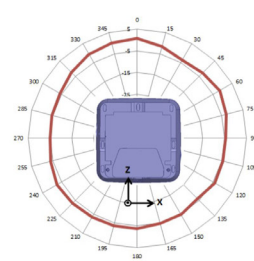
XZ-Ebene
