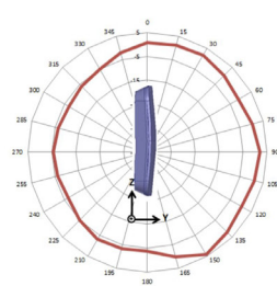
YZ-Ebene
